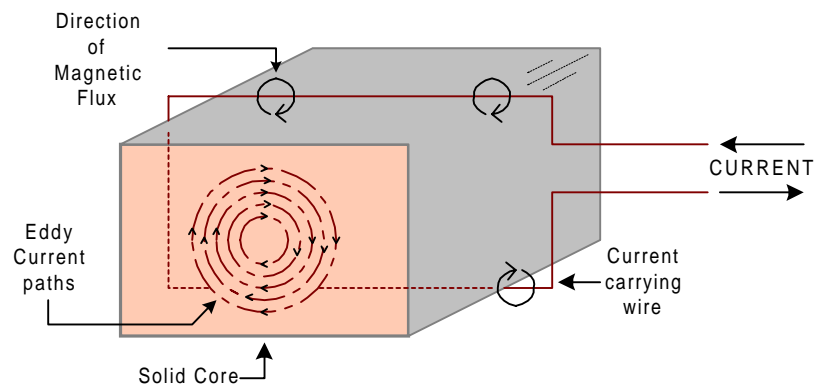
Figure 4: Eddy Currents induced in a solid iron core
