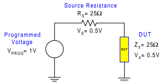
Figure 3: Constant Source Resistance
