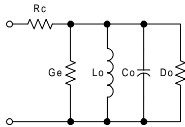
Equivalent Circuit: Air Core Inductor
