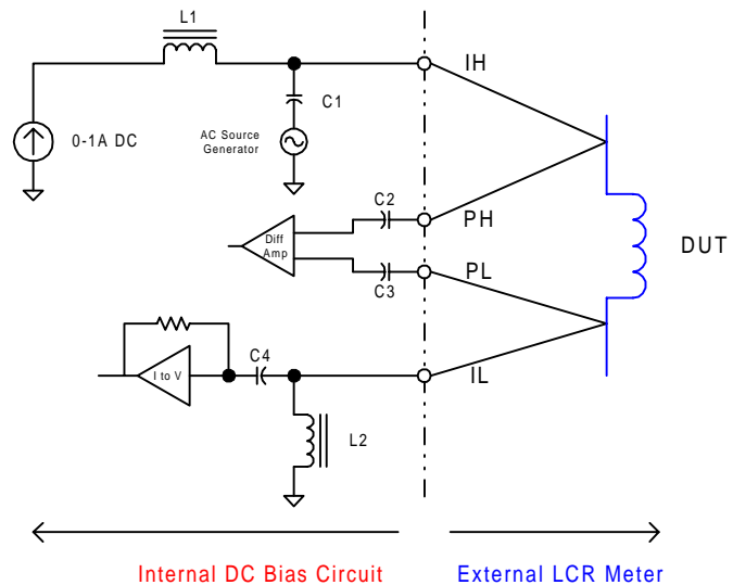
Figure 2: 1910 Internal DC Bias
