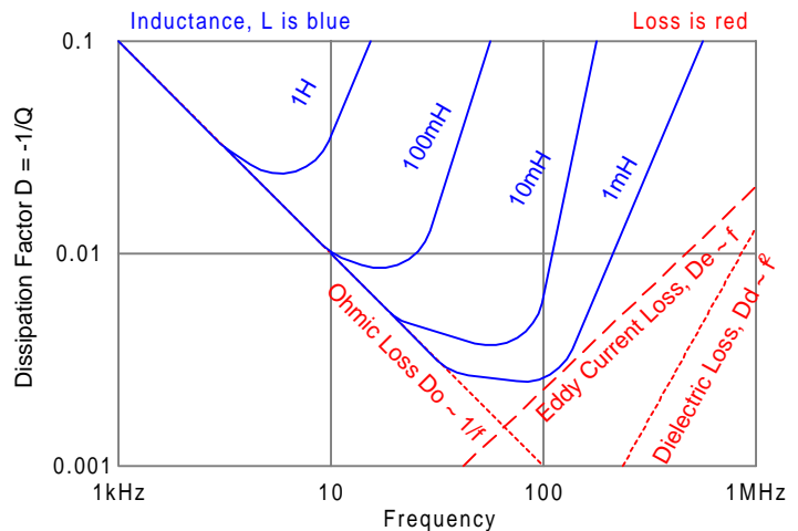
Figure 5: 1482 Inductance Standard Loss Curve
